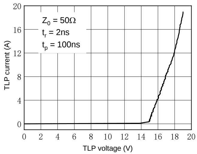
Fig7. TLP Measurement
