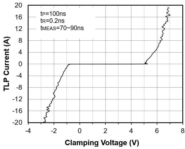
Fig7.TLP Measurement
