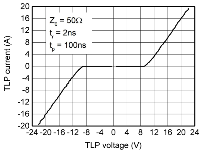
Fig.9 TLP Measurement
