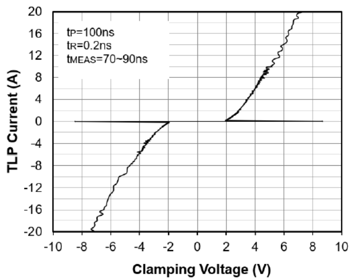
Fig7. TLP Measurement
