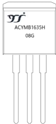
(TO-262-1 Package)
