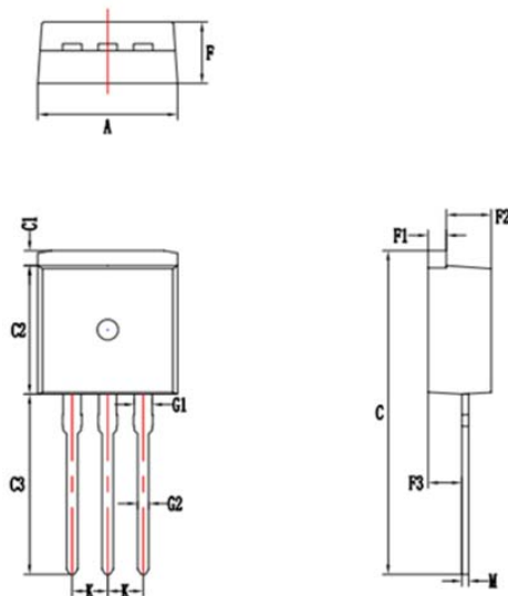
TO-262-1
