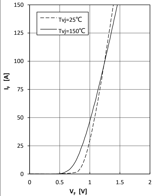
Fig14.Diode-Rectifier Forward Characteristics
